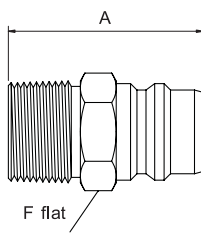
Plug
