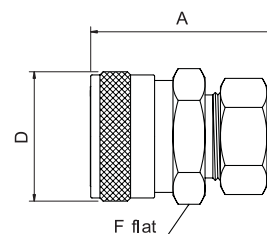
Body
